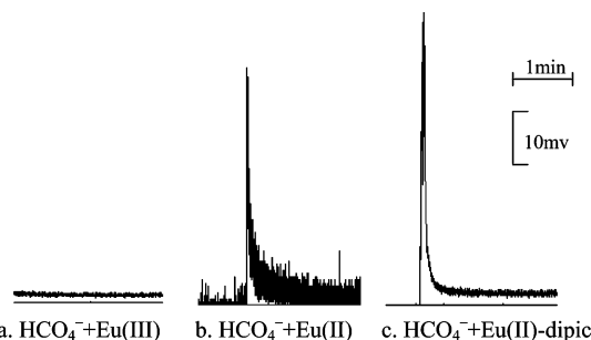
Figure 4. Chemiluminescence profiles in batch system. (a) Injection of 50 \mu\text{L} of 0.01 mol/L Eu(III) into the \text{HCO}_4^- solution; (b) injection of 50 \mu\text{L} 0.01 mol/L Eu(II) into the \text{HCO}_4^- solution; (c) injection of 50 \mu\text{L} 0.01 mol/L Eu(II)–dipicolinate complex into the \text{HCO}_4^- solution.
