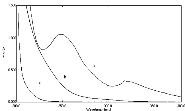
Figure 5. Absorption spectra of Eu(II) (a), Eu(II) after reaction (b), Eu(III) (c); concentration of all reagents: 1 \times 10^{-3} mol/L.
