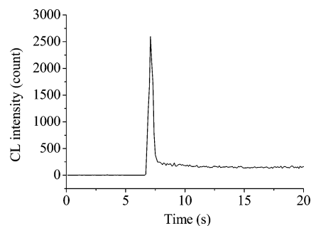
Figure 3. The CL kinetic curve of the system. Condition: injection 50 \mu\text{L} 0.01 mol/L Eu(II)–dipicolinate complex into \text{HCO}_4^- solution (2 mol/L \text{H}_2\text{O}_2 and 0.05 mol/L \text{HCO}_3^- were prepared 10 min prior to ensure the preequilibration of peroxy-monocarbonate formation).
