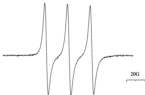
Figure 7. ESR spectrum of nitroxide radicals generated by reaction of the TEMP probe in \text{HCO}_4^- –Eu(II)–dipicolinate system. Conditions: receiver gain, 8.00 \times 10^4 ; mod amplitude, 1 G; sweep width, 100.00 G; microwave power, 3.17 \times 10^0 mW.
