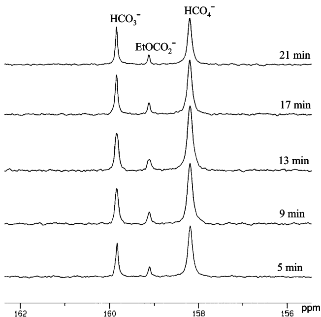
Figure 2. ^{13}\text{C} NMR spectra for a solution at 25 °C of \text{NaH}^{13}\text{CO}_3 (0.05 mol/L) in 1.76:1 (v/v) ethanol/water with [\text{H}_2\text{O}_2] = 2.0 mol/L. Times shown are for the completion of acquisition from the time of mixing.
