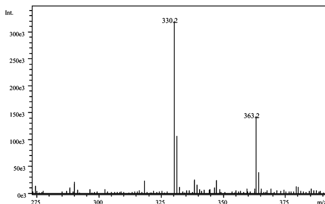
Figure 8. Mass spectra of DPA and DPAO 2 by chemical trapping with the DPA. 60 mmol/L DPA. Conditions: The reacted solution was placed for several minutes at room temperature, in a biphasic system composed of chloroform and \text{H}_2\text{O} (1:1, v/v) and protected from light.
