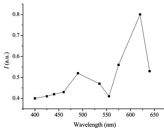
Figure 6. The CL spectral distribution for the system \text{HCO}_4^- -Eu(II)-dipicolinate with cutoff method.
