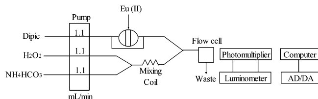
Figure 1. Schematic diagram of flow-injection CL detection system for (A) the on-line preparation of \text{HCO}_4^- solution; (B) the investigations of energy transfer CL.
